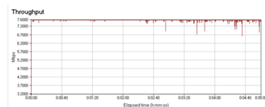
Figure 11 Throughput measurement
