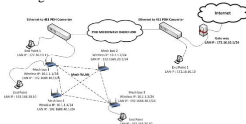
Figure 7. Mesh WLAN connected to internet gateway via Ethernet over PDH based radio link
