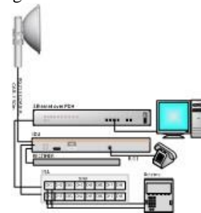
Figure 9. BER Measurement setup Table 4 BERtest result
